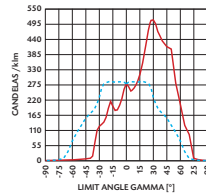
ASYMMETRIC REFLECTOR UMNA400H 400W E40
