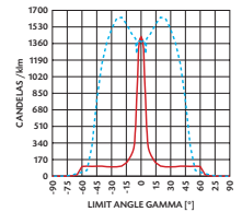
SPECULAR NARROW BEAM UMN400S 400W E40
