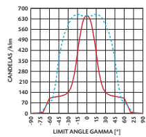
SYMMETRIC REFLECTOR UM400H 400W E40
